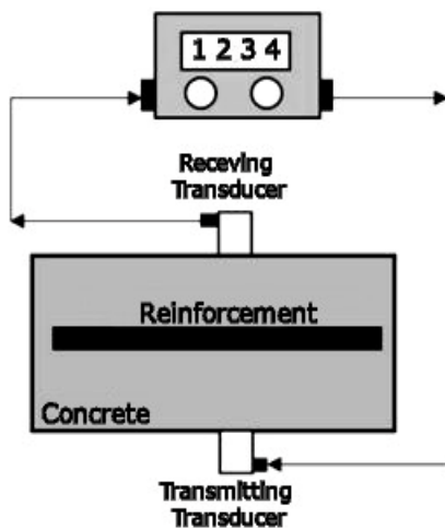
Figure 10: The principle of ultrasonic pulse velocity in civil engineering. [26]
