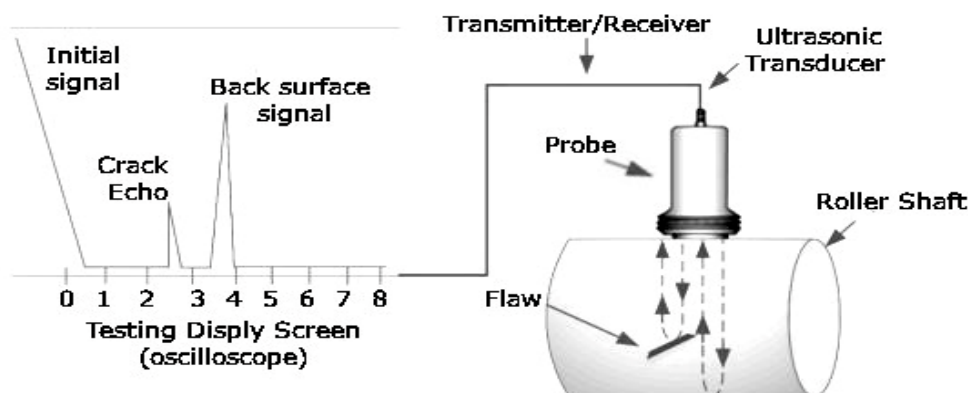
Figure 13: Illustration of ultrasonic testing (UT) set-up. [33]
