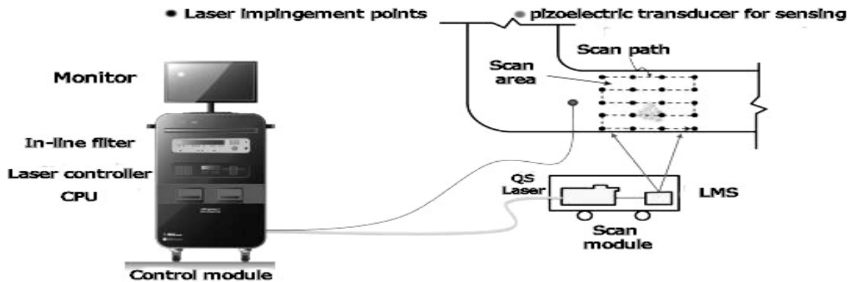
Figure 11: Ultrasonic propagation imager (UPI) for inspection of the nuclear power plant (NPP) pipeline (LMS: laser mirror scanner; CPU: central processing unit). [25]
