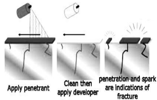
Figure 3: Illustration of Dye Penetrant Testing [6]
