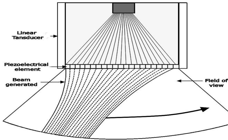
Figure 17: Diagram of linear ultrasound transducer - phased array. [52]
