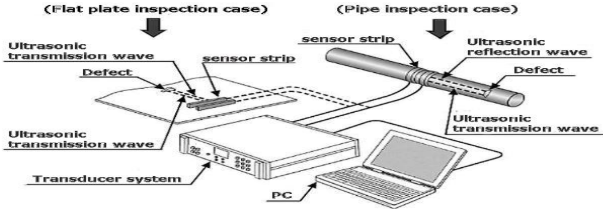
Figure 9: typical guided wave inspection system [16]
