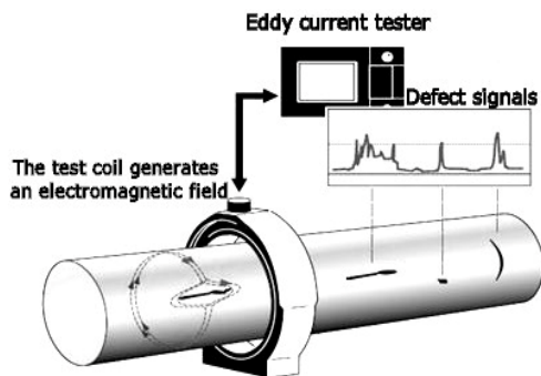
Figure 2: illustration of Eddy currents [5]
