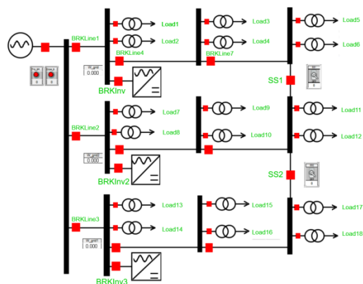
Figure 10. Microgrid model
