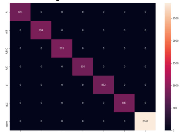
Figure 9. Confusion matrix
