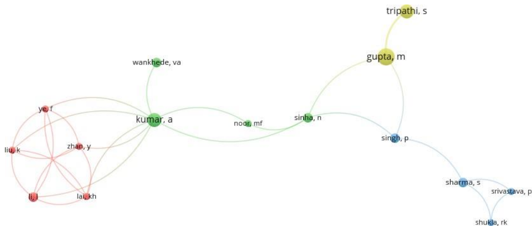
Figure 1. Co-citation map
